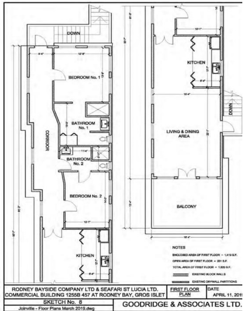
DIAGRAM A5.6 - PARCELS 457 - FIRST FLOOR PLAN
